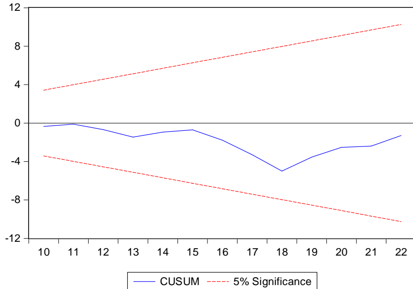
Figure 4.1: Post Estimation Diagnostic Test for Stability (CUSUM Test)
